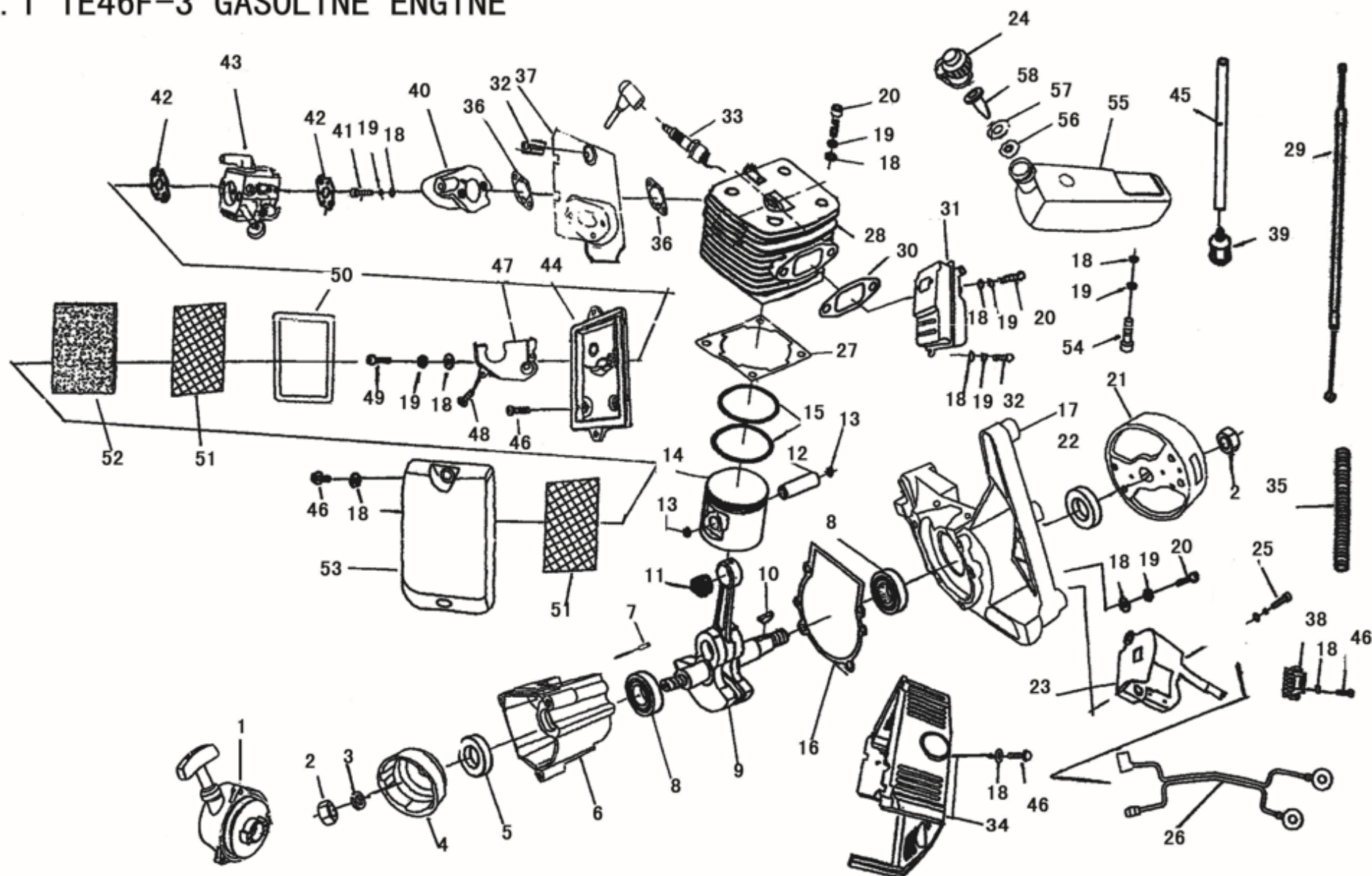
FIG. 1 1E46F-3 GASOLINE ENGINE
