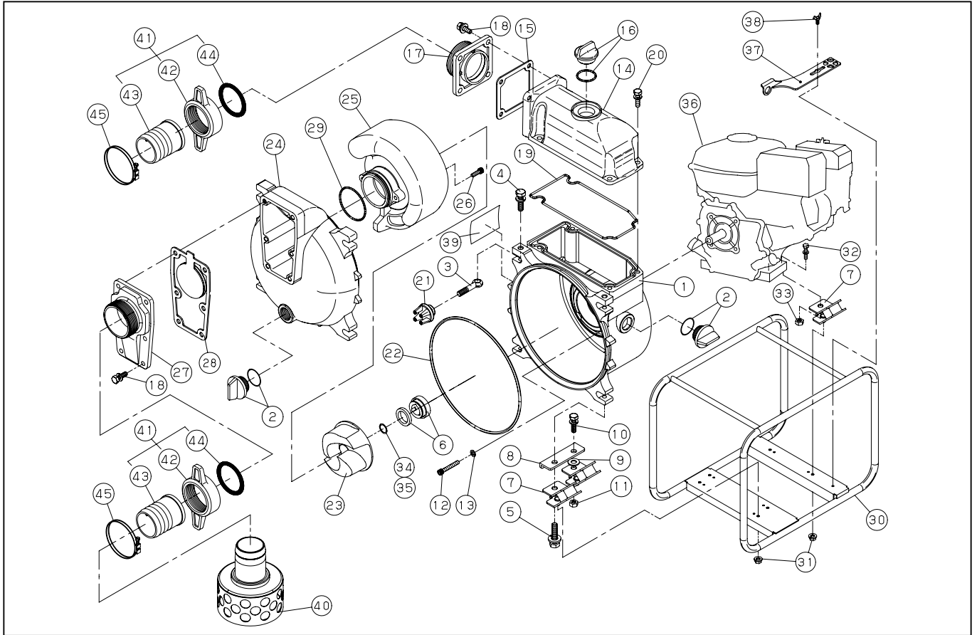
DWG No.012877804 MODEL : KTZ-100X FORM : KTZ-100X-BAF-0
