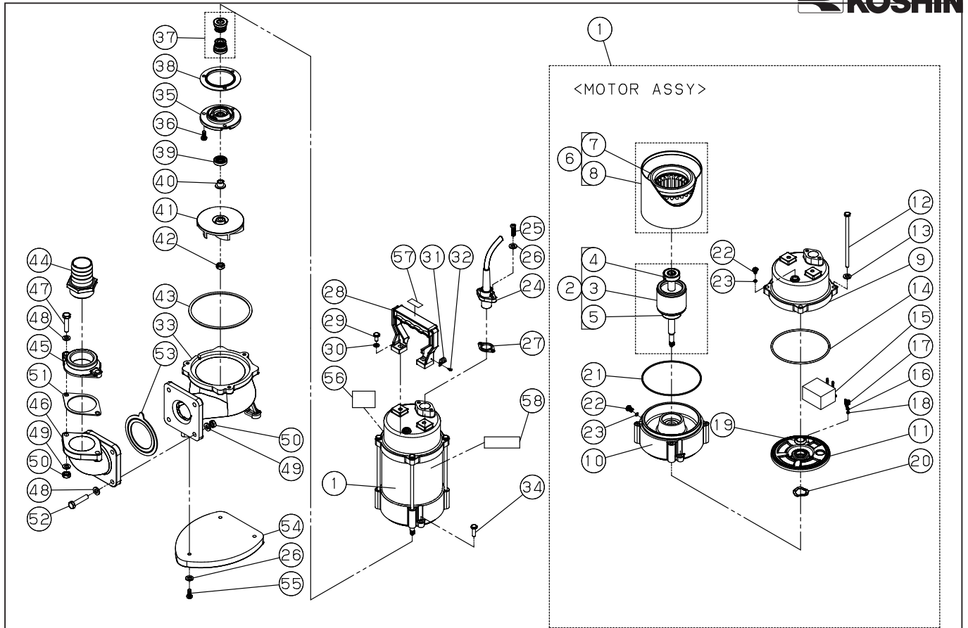
DWG No.077850701 MODELE : PKJ-400 FORM : PKJ-400-BAB-0
